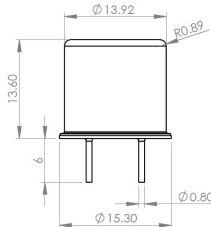
Pin-Side view
